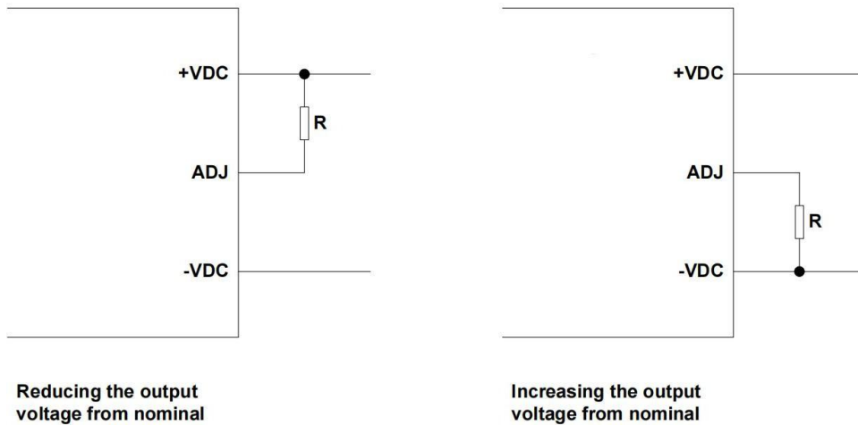
Figure 4: Output Adjustment
